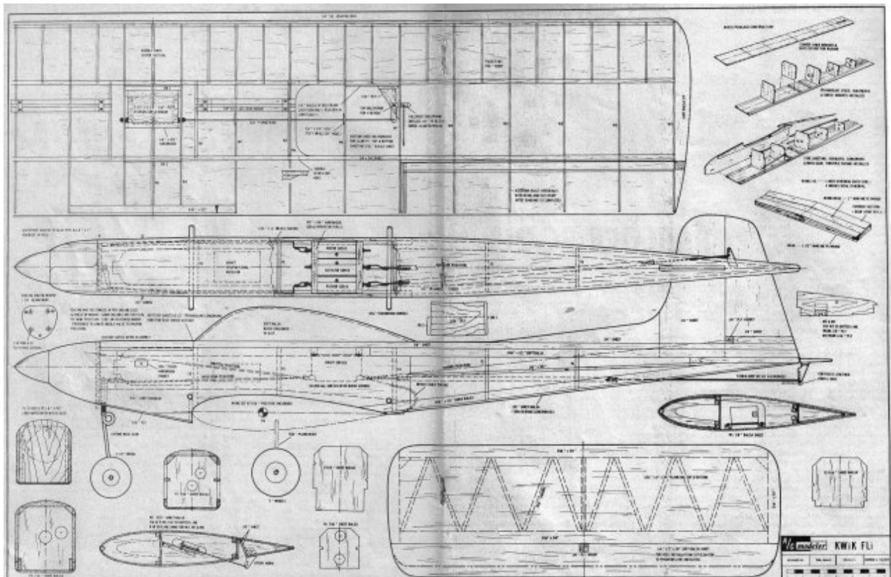
Kwik-Fli Mark I plan from Oct. 1964 RCM
