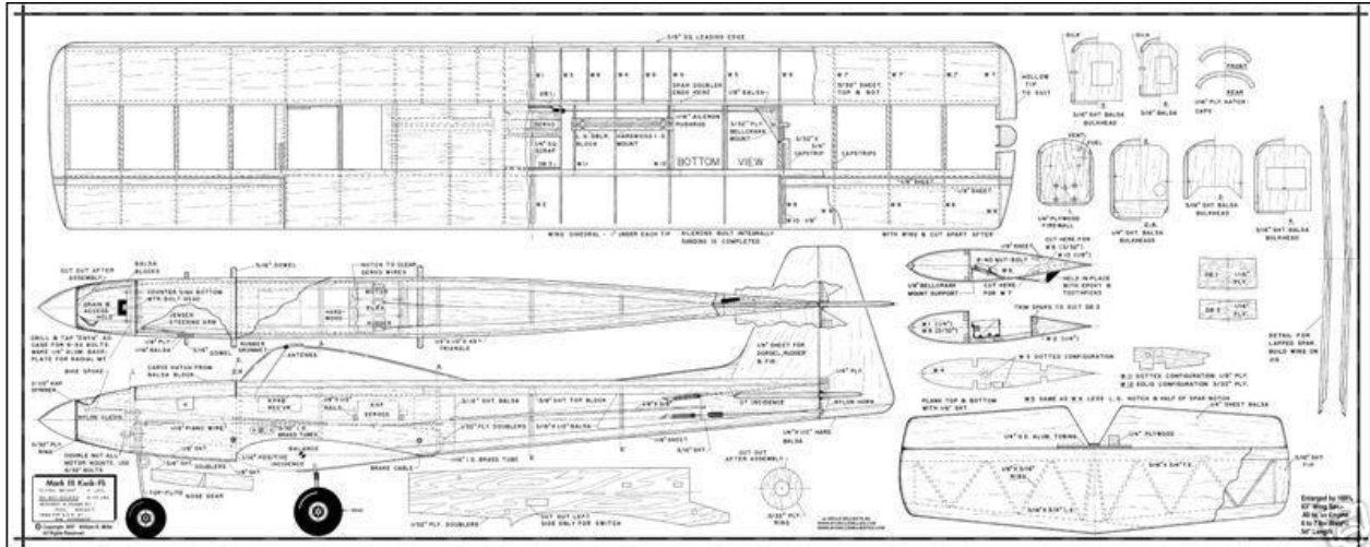
Kwik-Fli Mark III plan
